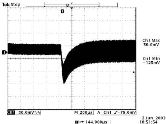
50% to 100% load transient at V_{in}=3.3 V, V_o=15 V
